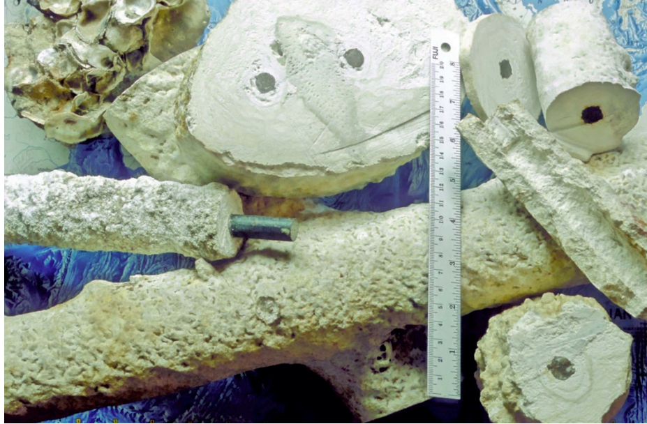
Two years of Biorock material growing on iron bar. Photo Wolf Hilbertz.
